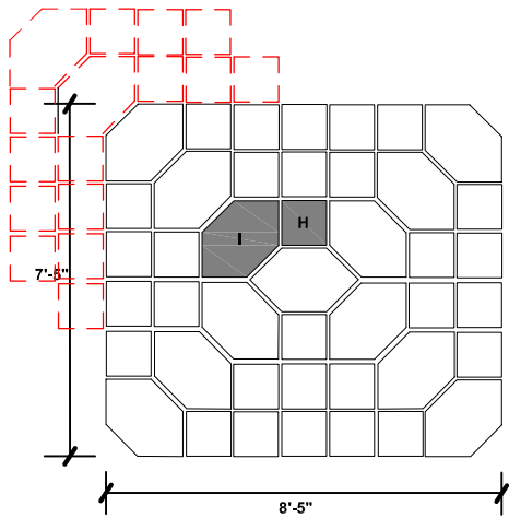
STANDARD DIAMOND KIT PATTERNS SQ FT= APPROX. 62.5 SQ FT
