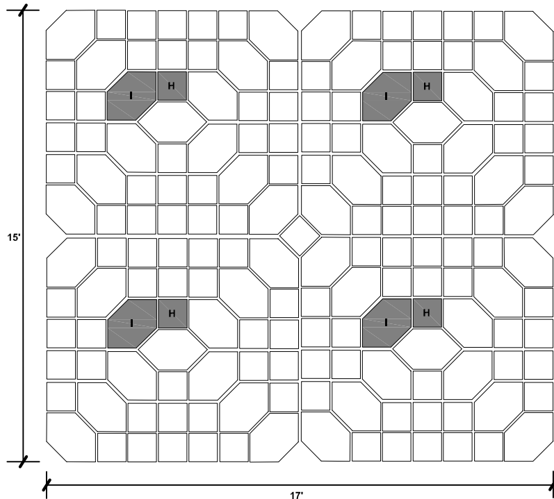
PATIO (4 KITS JOINED) PATTERNS SQ FT= APPROX. 255 SQ FT
